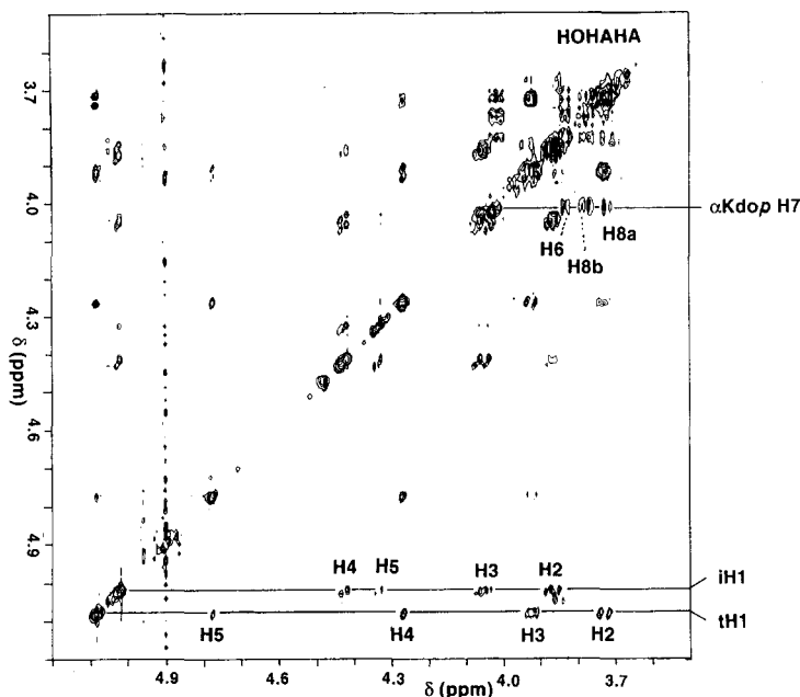
Fig. 3. Partial 2D HOHAHA spectrum of fraction M1.
