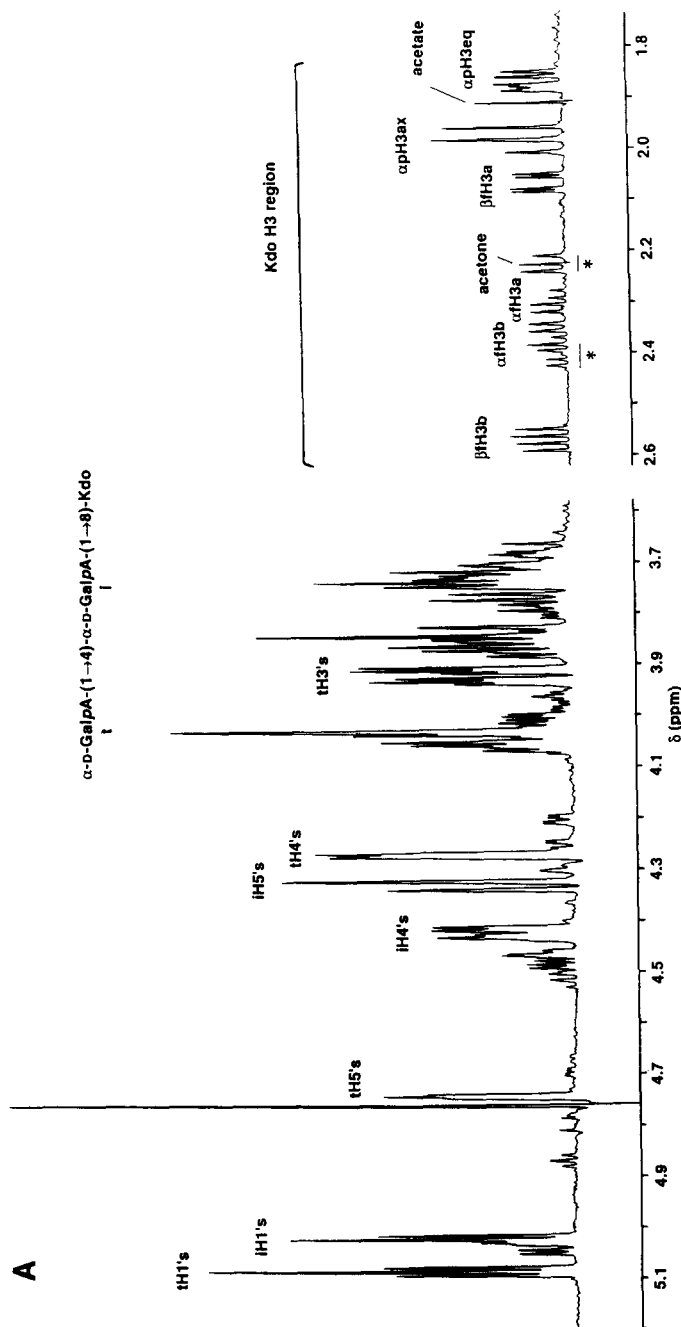
Fig. 2. 500-MHz ^1\text{H} NMR spectra of A, fraction M1 and B, fraction M2 in \text{D}_2\text{O} . In the spectrum of M1, the coupled signals marked with an asterisk at \delta 2.402 (doublet of doublets) and 2.223 (doublet) could not be explained so far.
